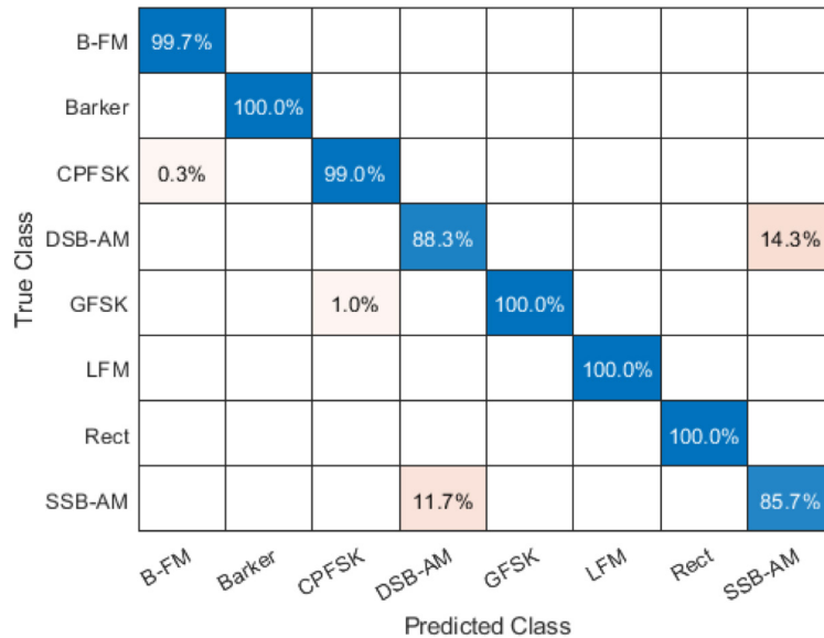
Figure 5. Confusion matrix with the results of the classification.
