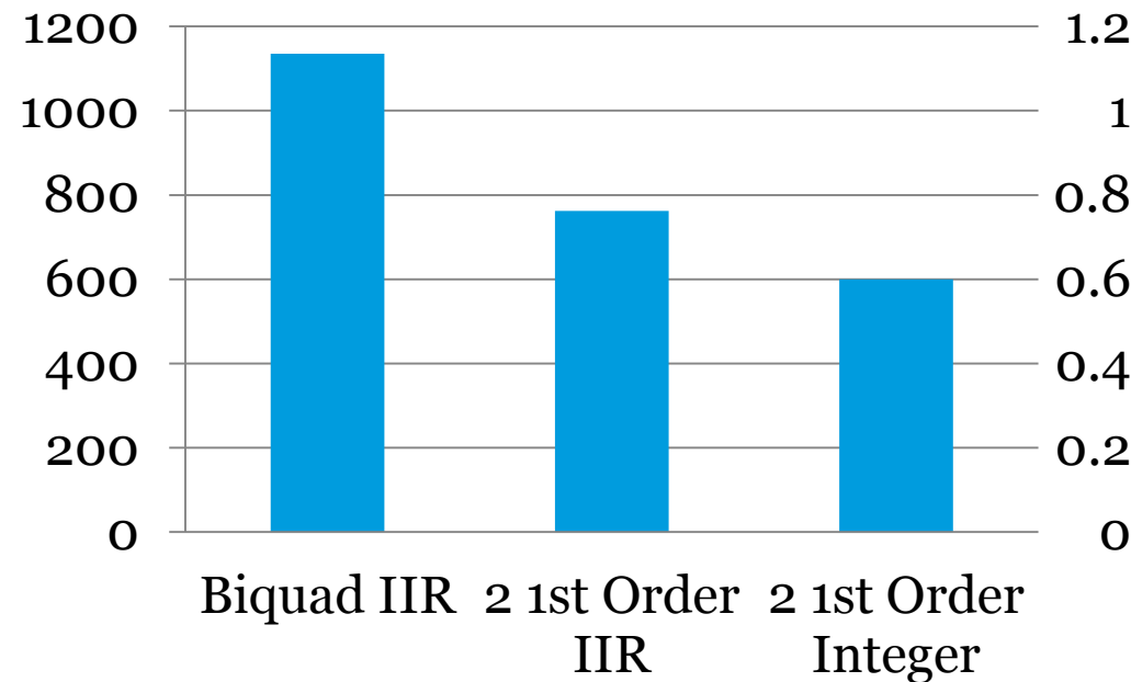
Energy (nW/MHz)
